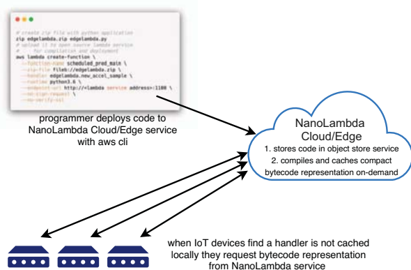
Fig. 2. Life cycle of a function deployment from the application developer’s command line to the NanoLambda Cloud/Edge service to the IoT device running NanoLambda On Device
