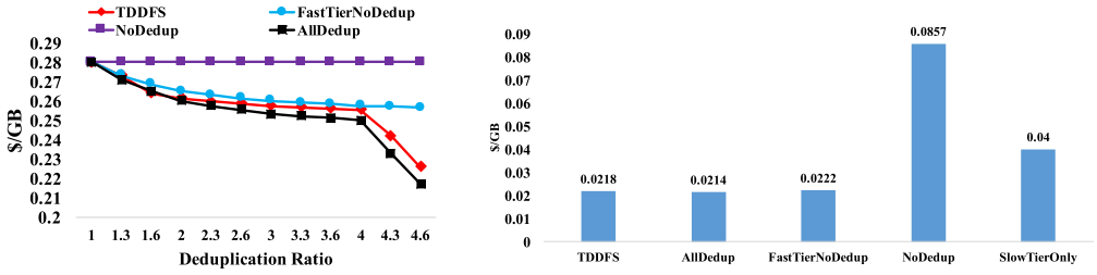
(a) $/GB comparison of TDDFS, NoDedup , AllDedup , and FastTierNoDedup with different deduplication ratios
