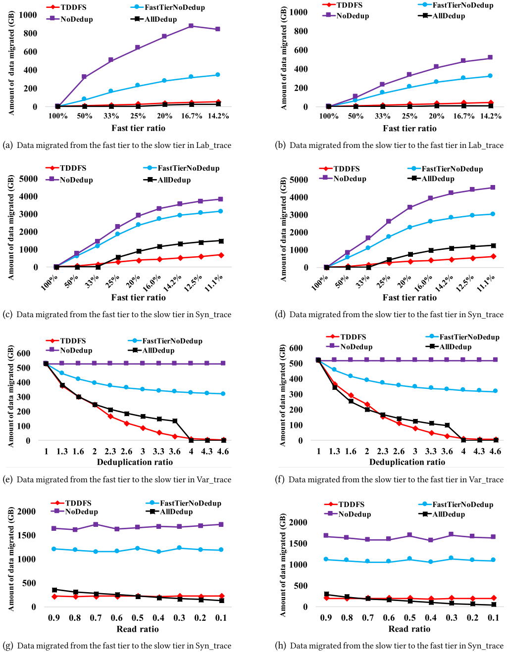
Fig. 6. Migration cost comparison of TDDFS, NoDedup, AllDedup, and FastTierNoDedup.
