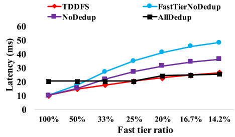
(b) Latency of Lab_trace
