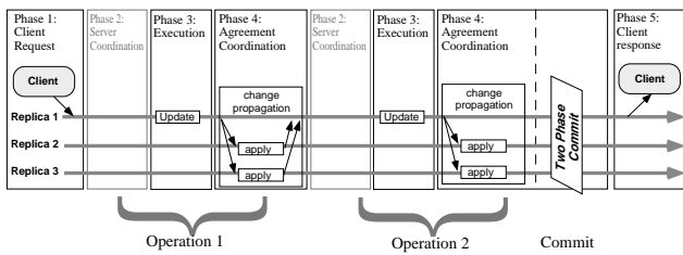
Figure 11. Eager primary copy approach for transactions
