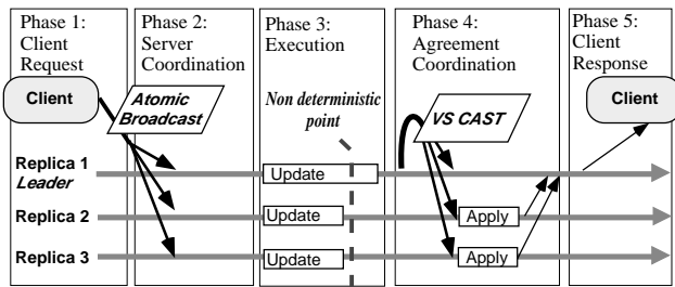
Figure 4. Semi-active replication
